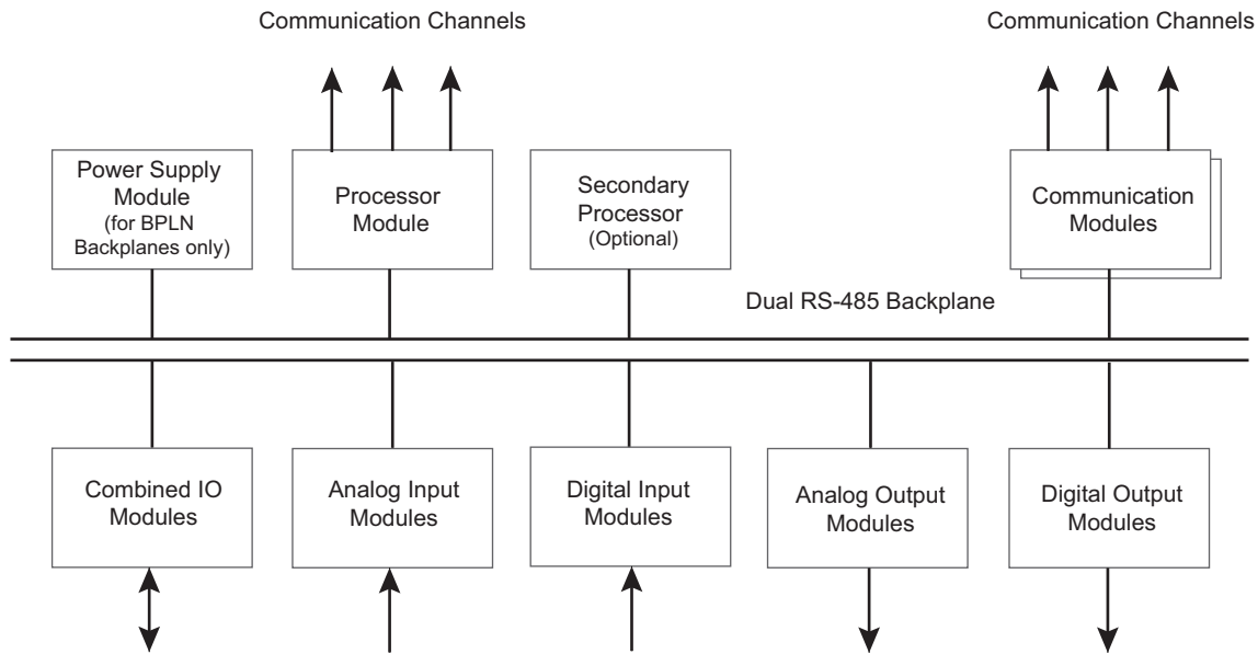
Figure 2. SCD2200 Bus Architecture
