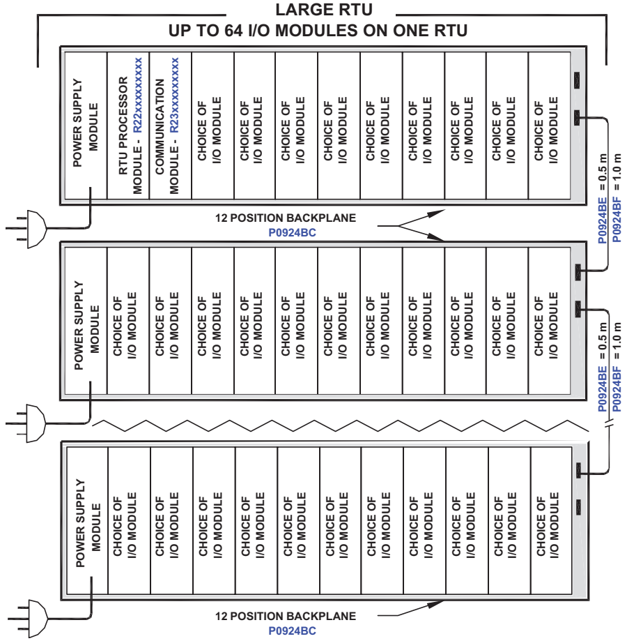
Figure 9. Large RTU with BPLN Backplanes
