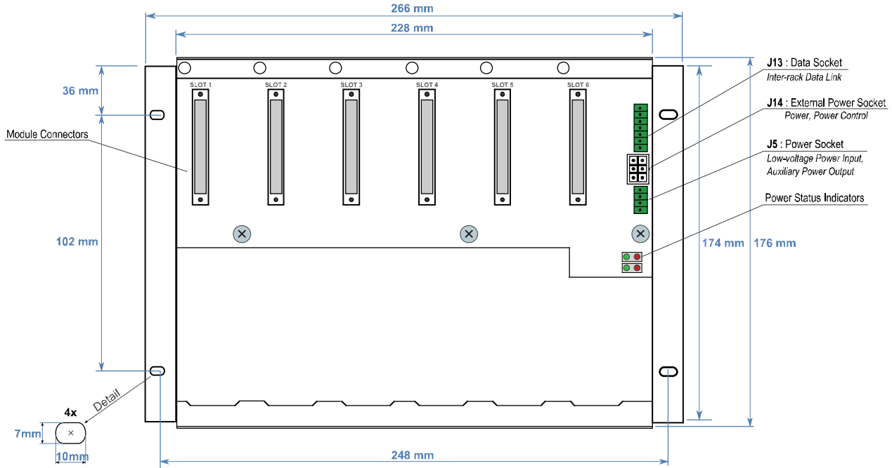
Figure 19. 6-Slot Integrated-power Backplane
