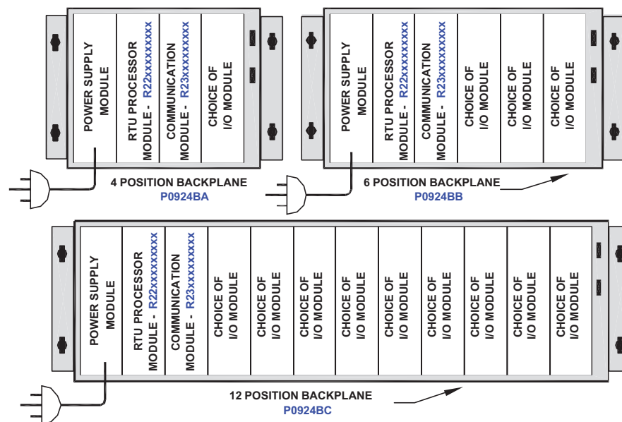
Figure 8. BPLN Backplane Module Layouts
