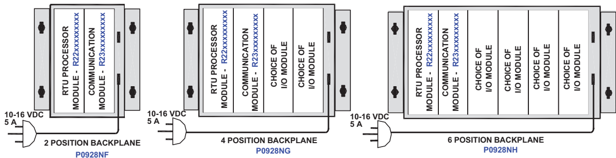
Figure 11. BP-x Backplane Module Layouts
