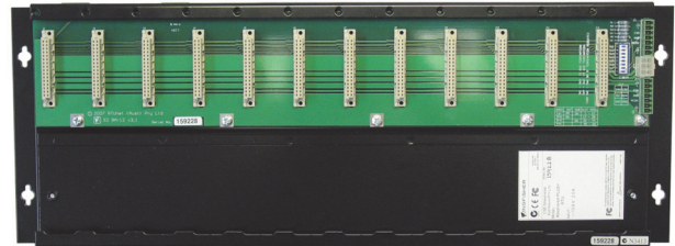
Figure 7. Empty 12-Slot Backplane
