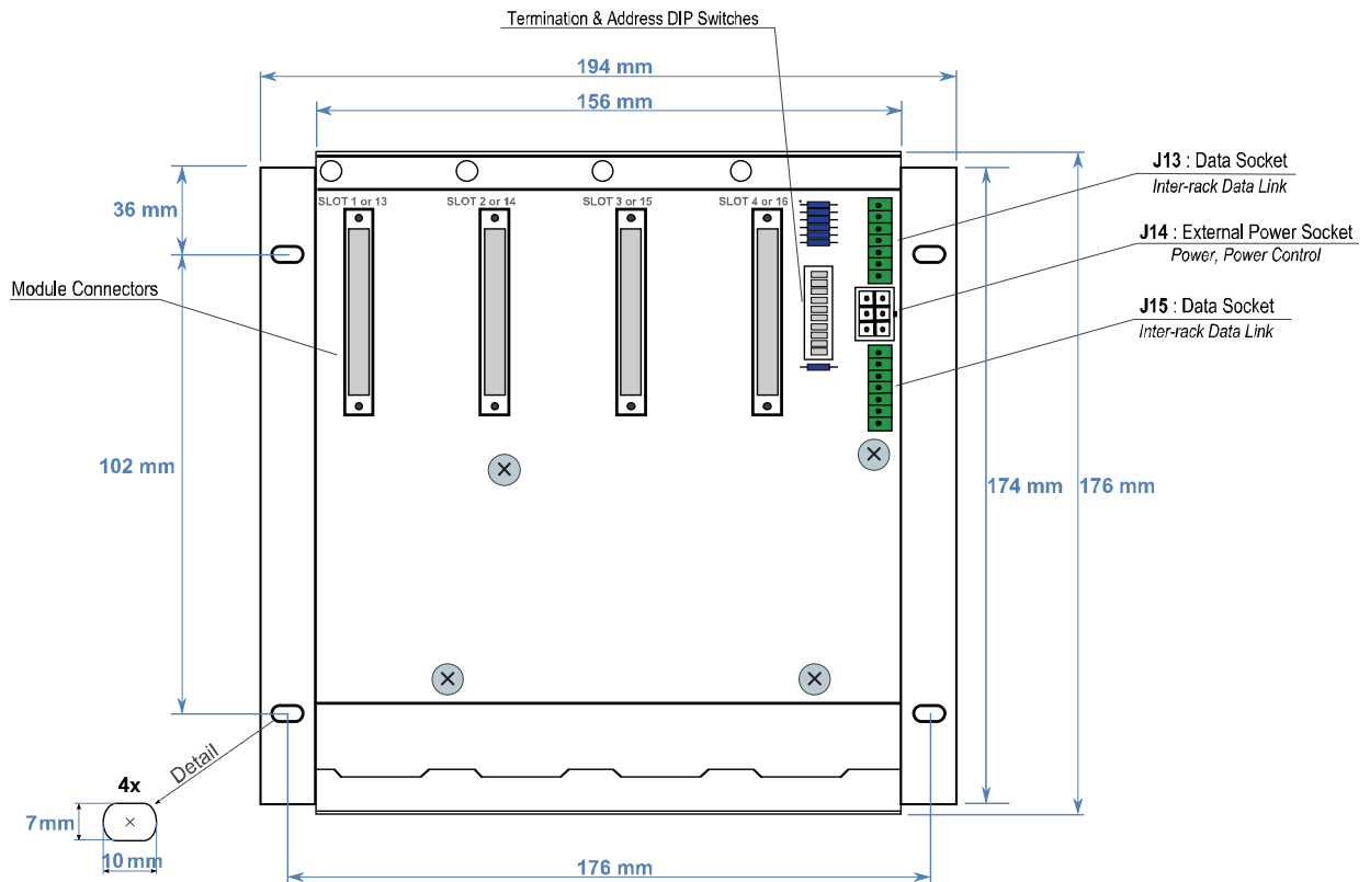
Figure 14. 4-Slot Passive Backplane
