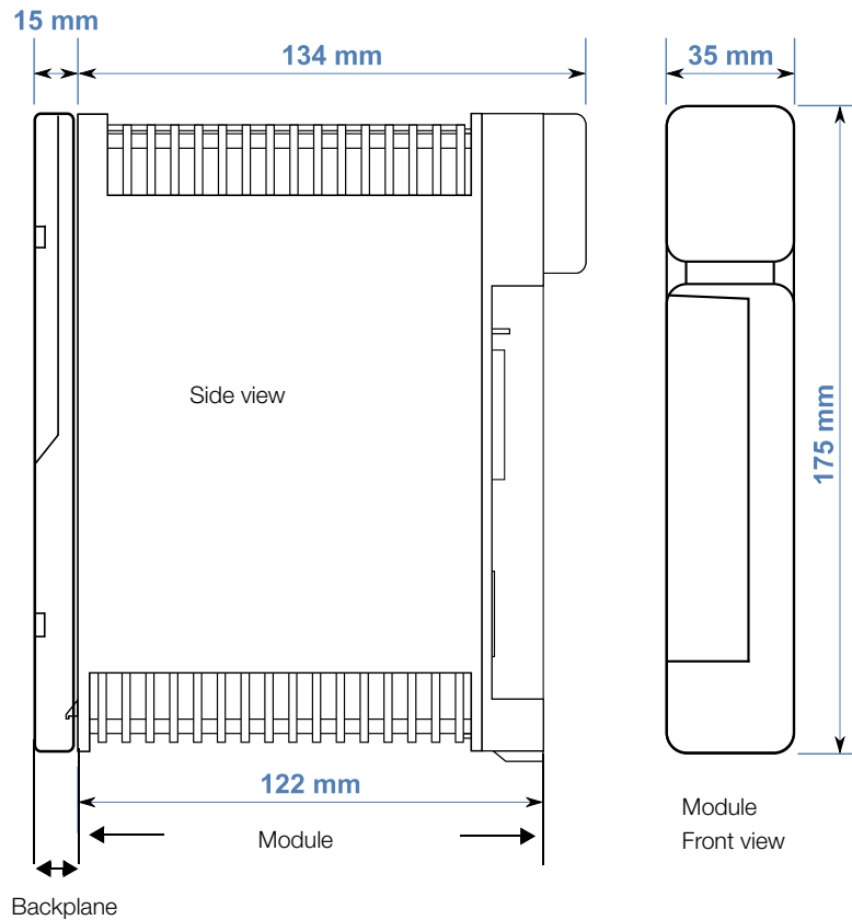
Figure 13. Module Mounted on a Backplane
