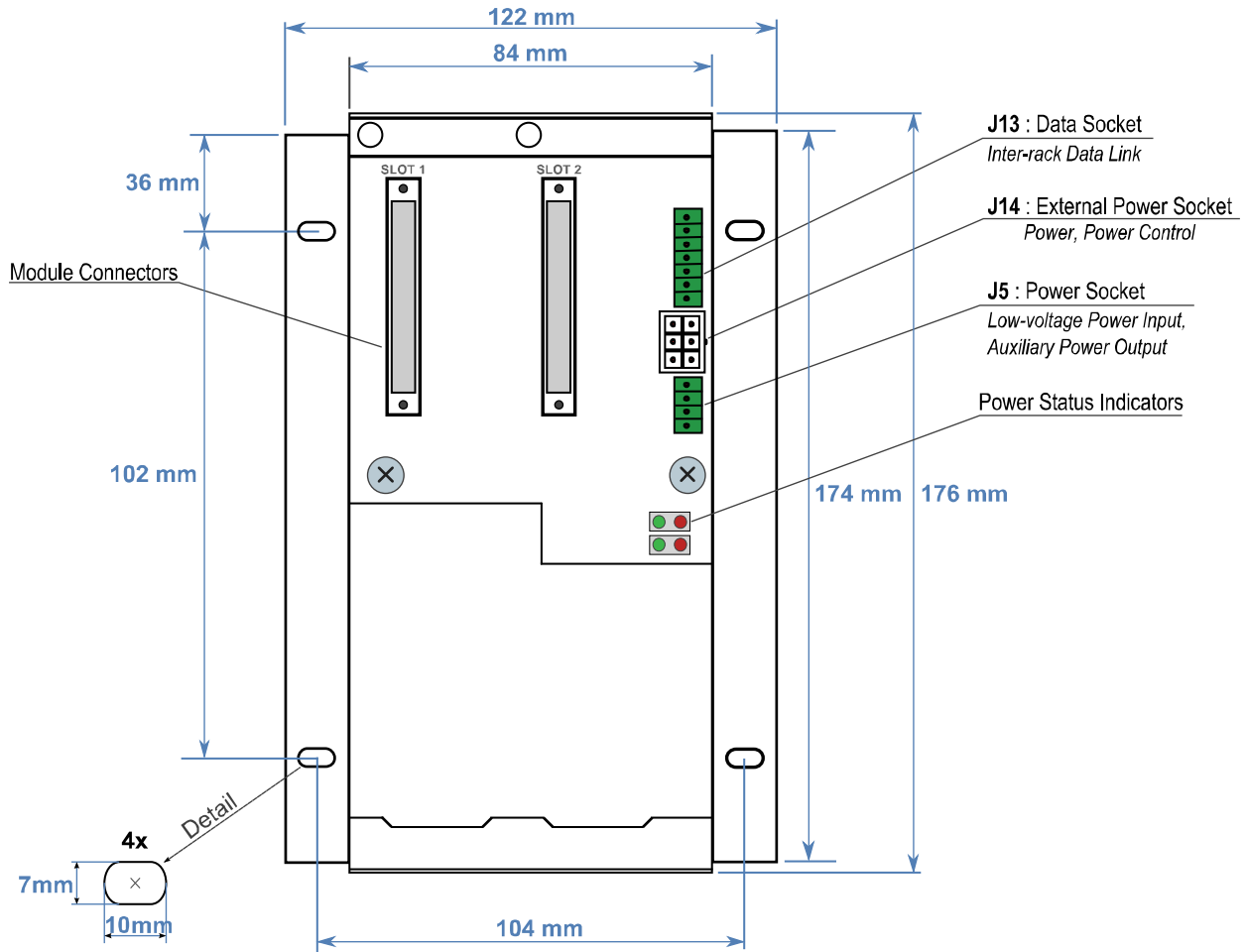
Figure 17. 2-Slot Integrated-power Backplane
