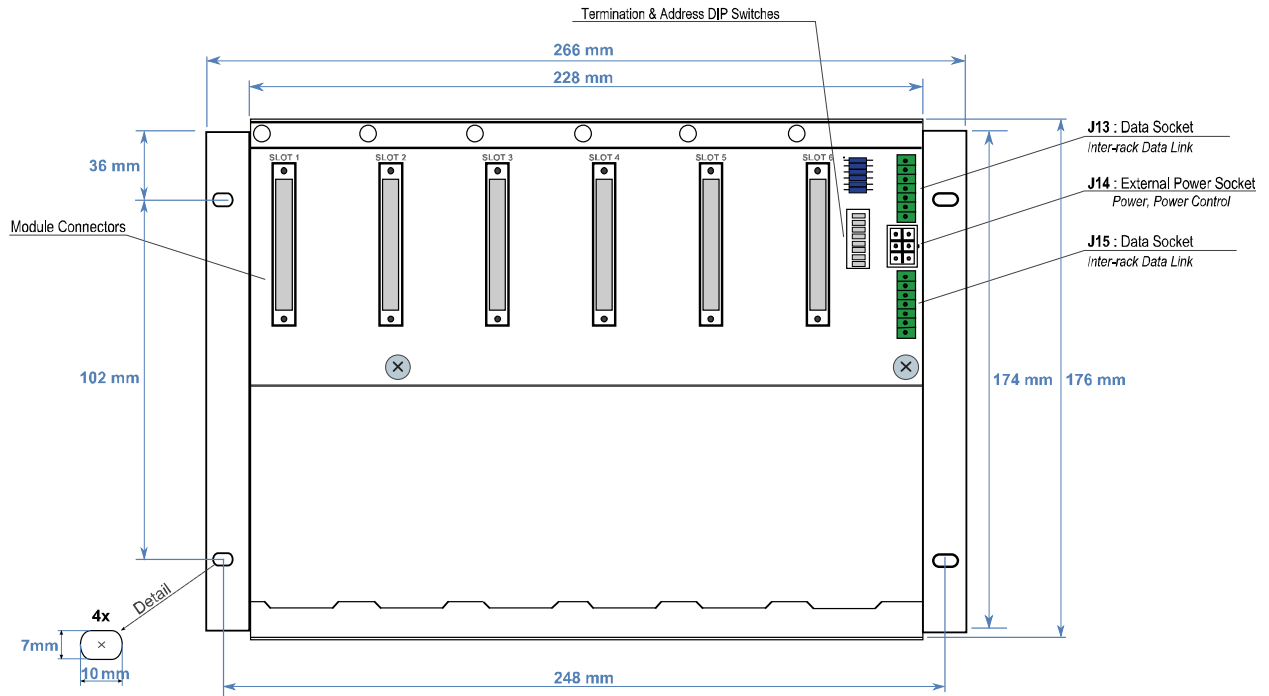
Figure 15. 6-Slot Passive Backplane
