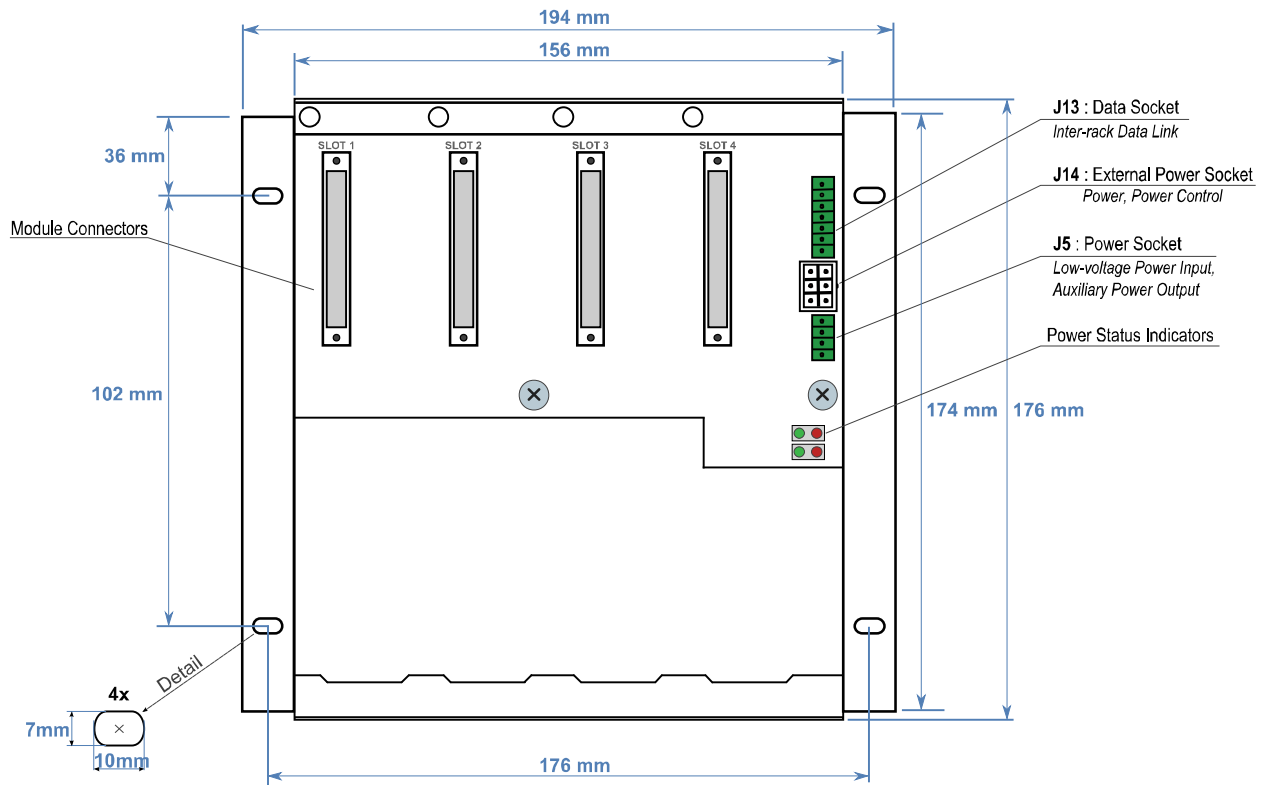
Figure 18. 4-Slot Integrated-power Backplane
