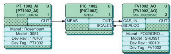
Figure 3. Block Diagram Typical CIH Loop
