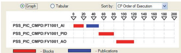
Figure 2. Schedule for Single CIF Loop
