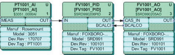
Figure 1. Block Diagram Typical CIF Loop
