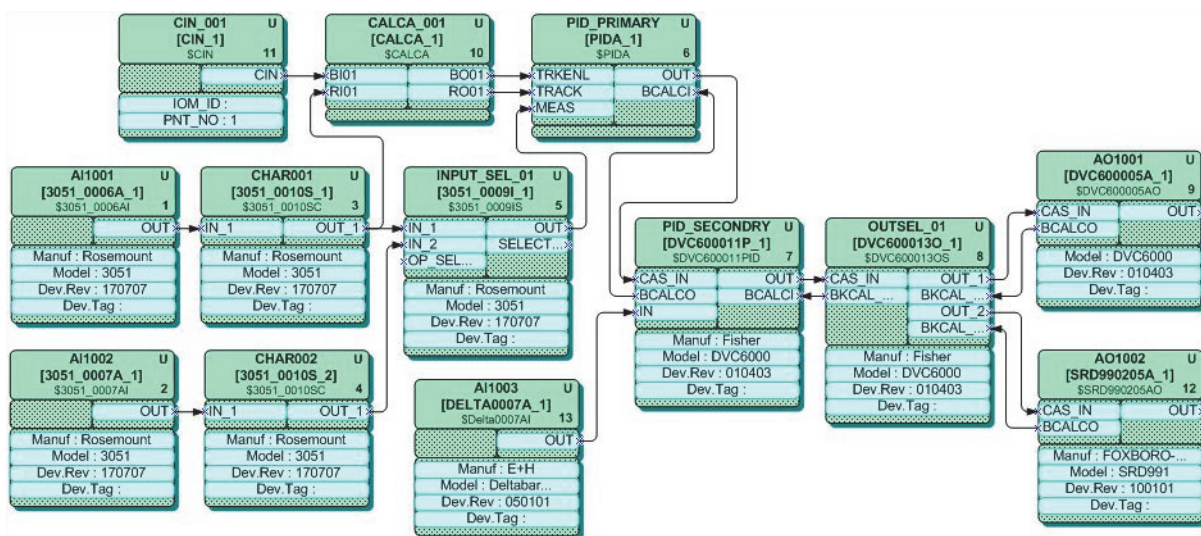
Figure 4. Typical Mixed CIH and CIF loop
