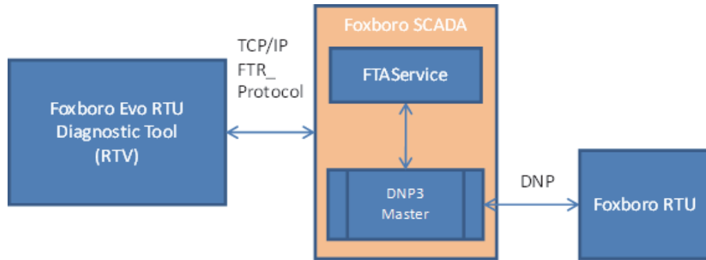
Figure 4. Remote Configuration of RTU over Serial Line
