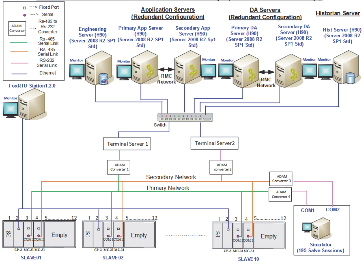
Figure 7. Foxboro SCADA with 200 DNP3 slaves (RTUs) in Serial Multi-drop Connection
