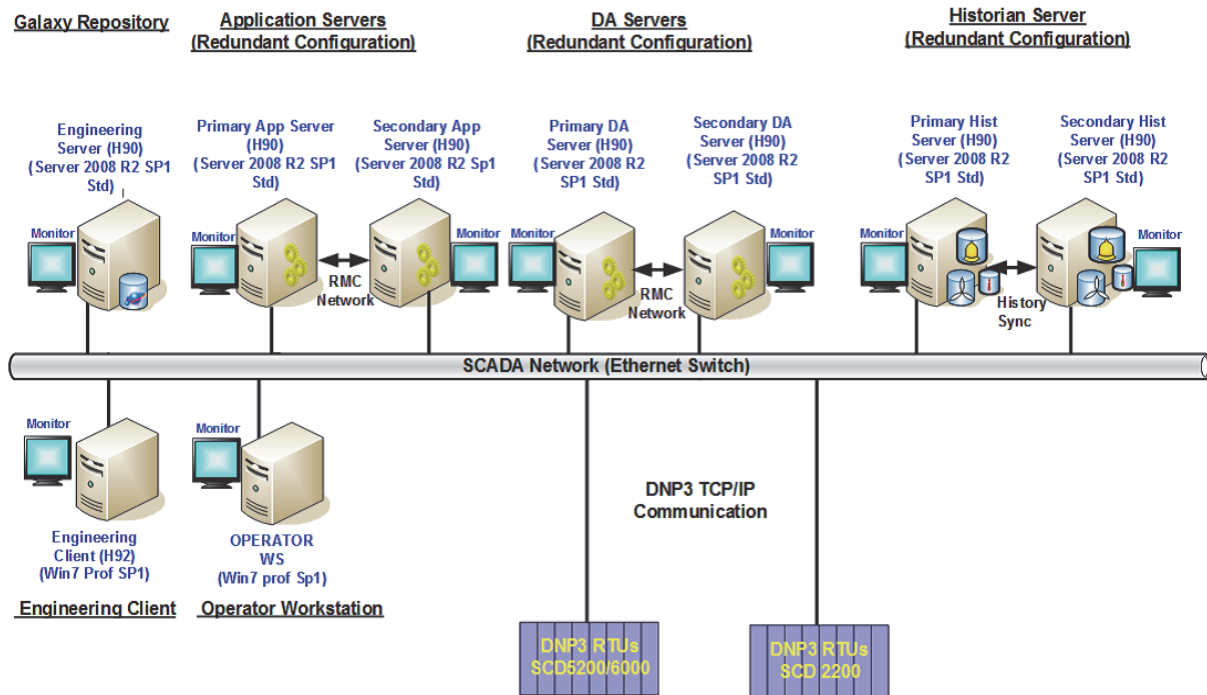
Figure 5. Foxboro SCADA with 80 DNP3 Slaves (RTUs) over TCP/IP - Physical Setup
