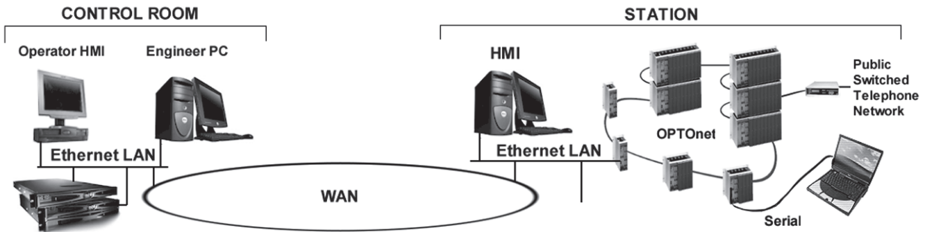
Figure 1. RTV to SCD5200 Communications Options
