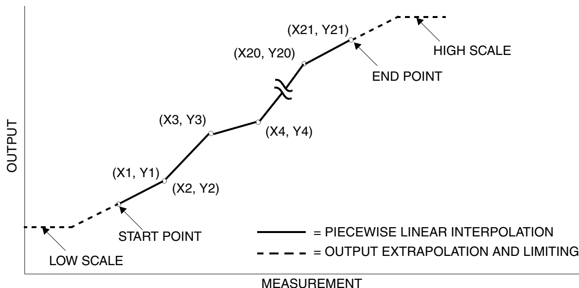
Figure 1. Characterization Curve
