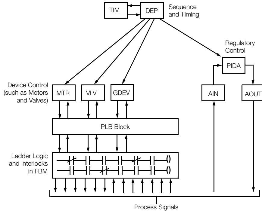
Figure 1. Total Integration of Foxboro Evo Control Software in a Single Control Processor
