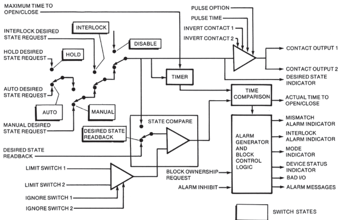
Figure 1. GDEV Simplified Signal Flow Diagram
