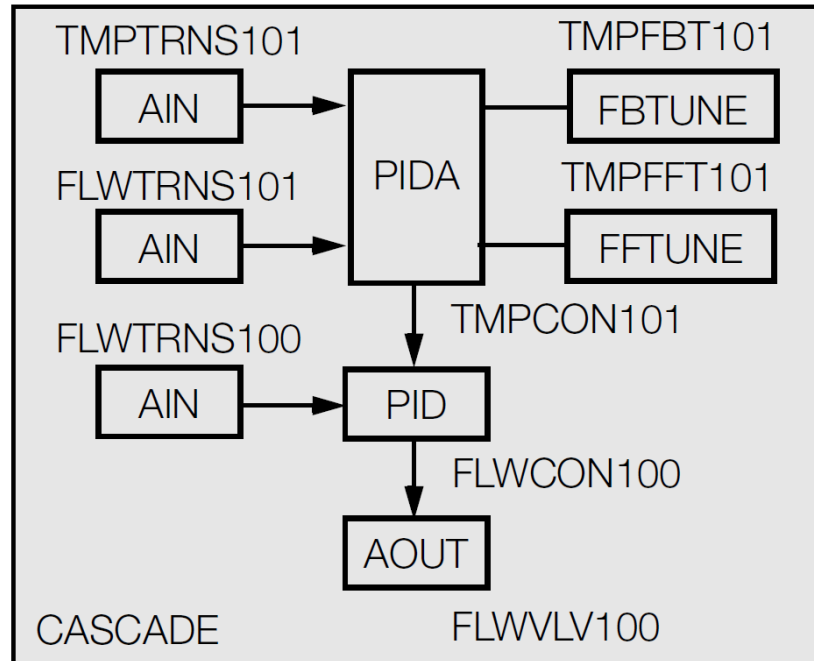
Figure 3. Example of a Cascade Control Strategy
