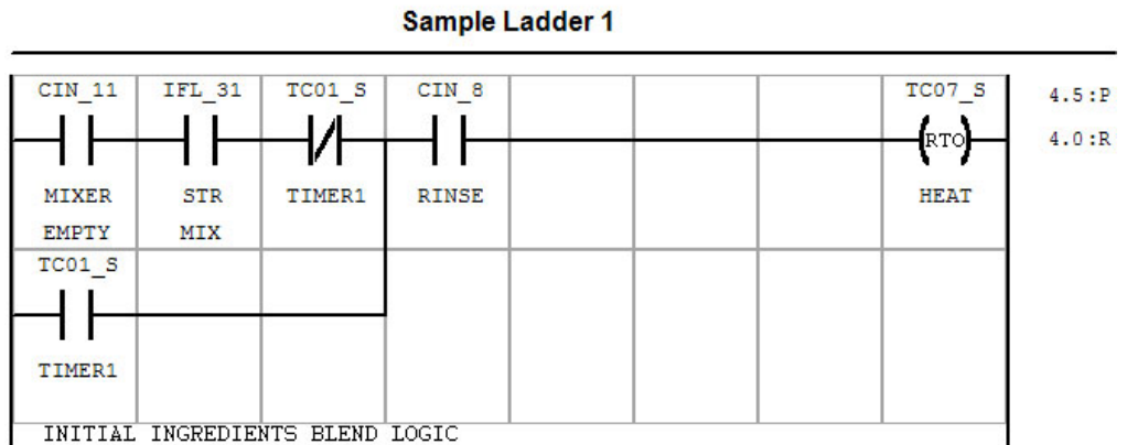
Figure 4. Sample Ladder Diagram
