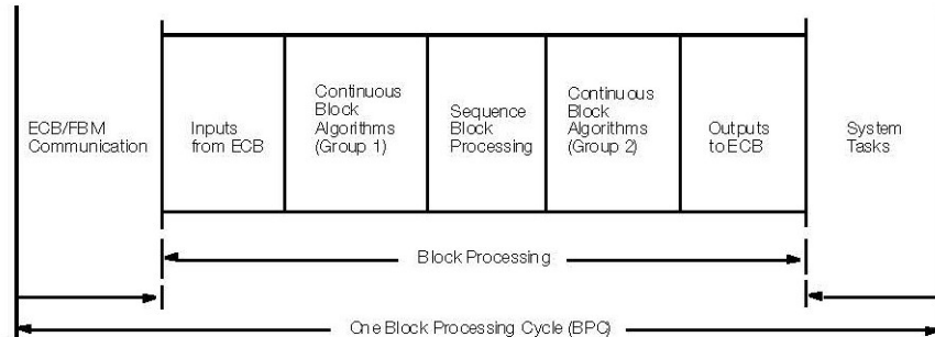
Figure 2. Block Processing Cycle (BPC)
