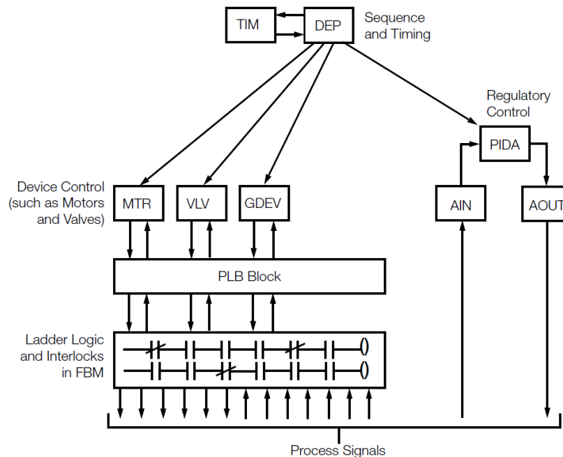
Figure 1. Total Integration of Foxboro DCS Control Software in a Single Control Processor
