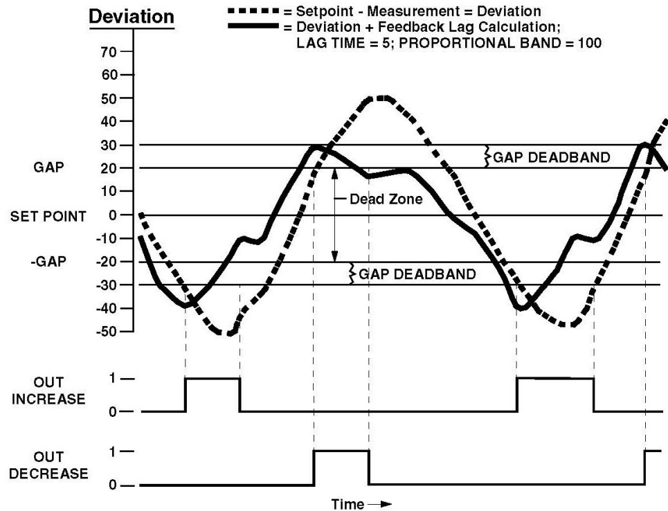
Figure 3. Feedback Lag Algorithm Timing Diagram
