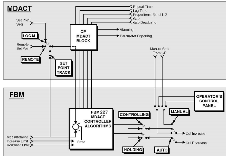
Figure 1. MDACT Simplified Signal Flow Diagram
