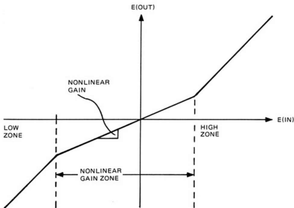
Figure 1. Nonlinear Gain Characteristics
