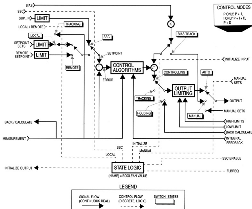
Figure 2. PIDX Block, Simplified Diagram
