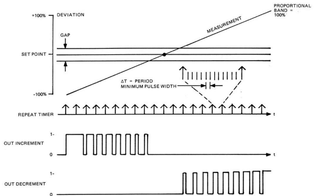
Figure 2. Pulse Duration Algorithm Timing Diagram
