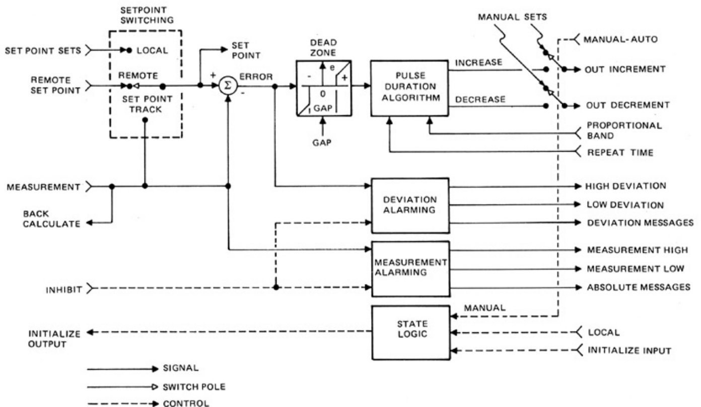
Figure 1. PTC Signal Flow Block Diagram
