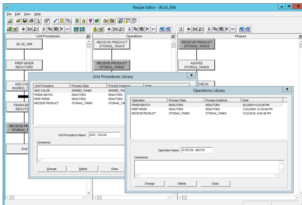
Figure 1 - Batch Recipe Structure
