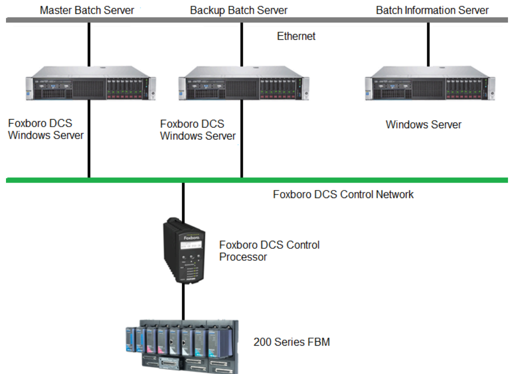
Figure 9 - Batch Server Redundancy
