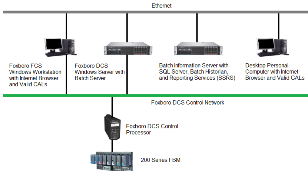
Figure 11 - Batch Reporting System Configuration
