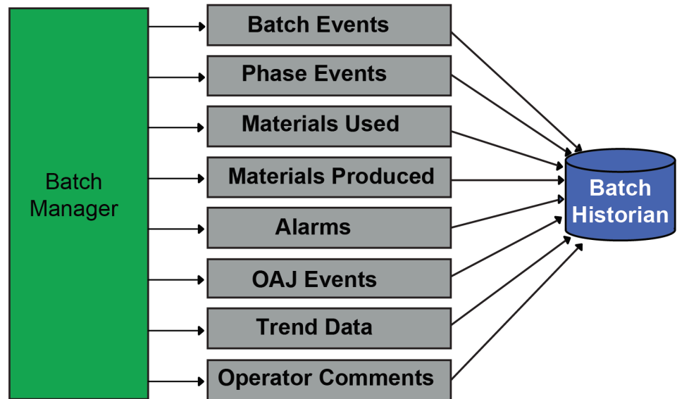
Figure 3 - Batch History (EBR)
