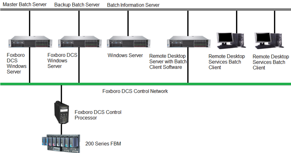
Figure 10 - Batch Management Software and Remote Desktop Services
