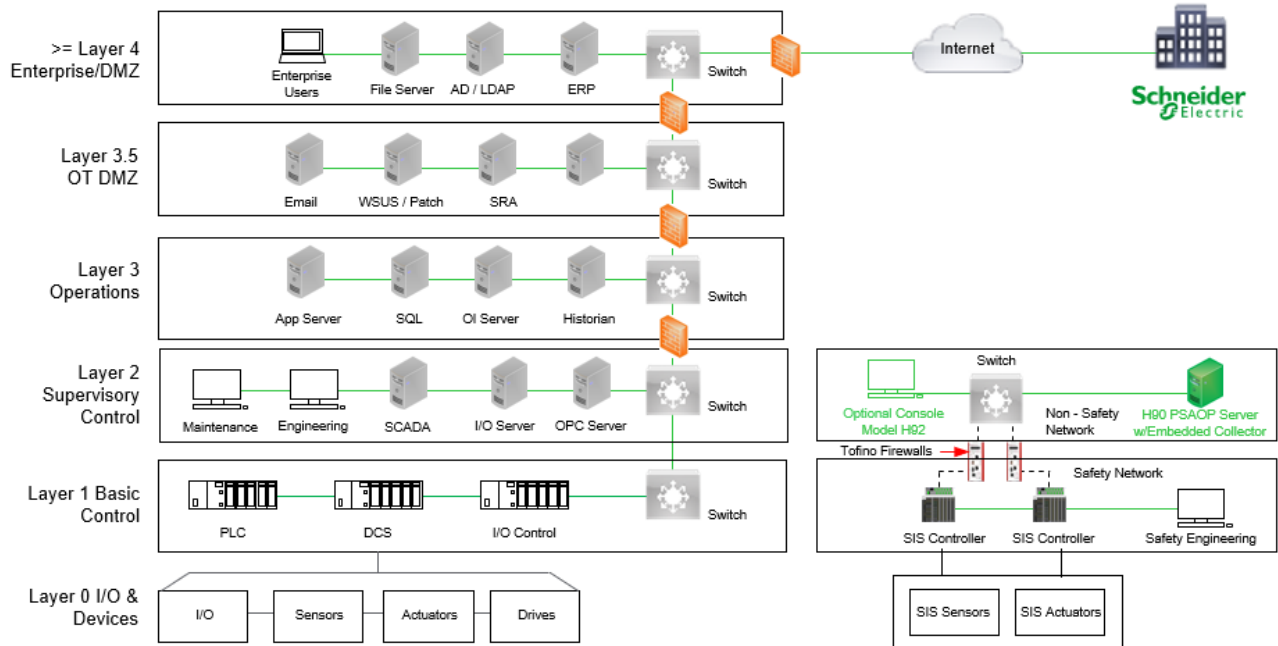
Figure 11 - Isolated (Air Gapped) Architecture for Small and Medium Systems – H90 All-in-one Server, H92 Console
